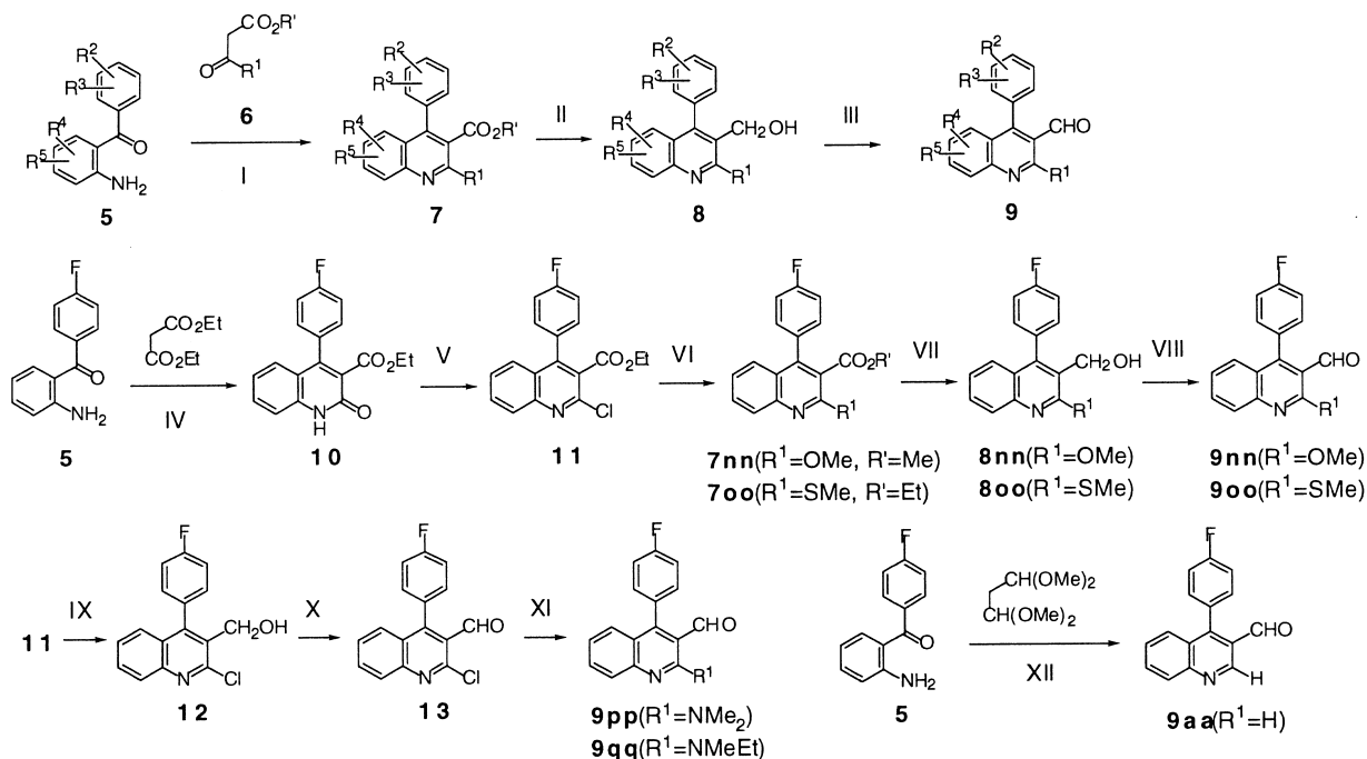
Scheme 1. Synthesis of 9 . Reagents and conditions: (I) H_2SO_4 , AcOH, reflux or methanesulfonic acid, benzene, reflux; (II) DIBALH, toluene, -25^\circ C ; (III) PCC, AcONa, CH_2Cl_2 , rt; (IV) piperidine, reflux; (V) POCl_3 , reflux; (VI) 7nn Na, MeOH, rt; 7oo MeSNa aq, THF, MeOH, reflux; (VII) 8nn : DIBALH, toluene, -40^\circ C ; 8oo : DIBALH, toluene, -75^\circ C ; (VIII) DMSO, (COCl)_2 , Et_3N , CH_2Cl_2 , -78^\circ C ; (IX) DIBALH, CH_2Cl_2 , -78^\circ C ; (X) DMSO, (COCl)_2 , Et_3N , CH_2Cl_2 , -78^\circ C ; (XI) amine, toluene, 140^\circ C in autoclave; (XII) ZnCl_2 , toluene, reflux.
