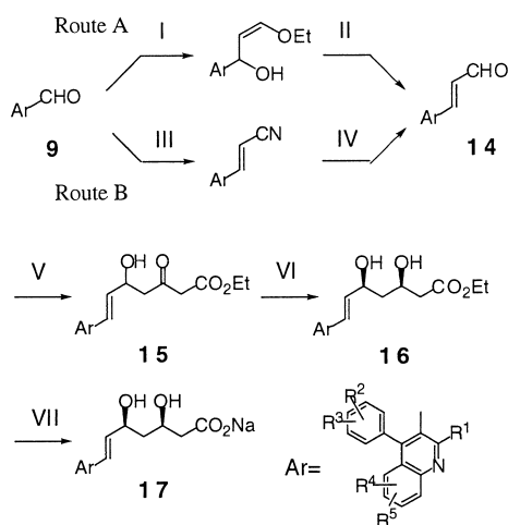
Scheme 2. Synthesis of 17 . Reagents and conditions: (I) n\text{-Bu}_3\text{SnCH=CHOEt} , n\text{-Buli} , THF, -78^\circ\text{C} ; (II): PTS, THF, \text{H}_2\text{O} , rt; (III): (\text{EtO})_2\text{POCH}_2\text{CN} , \text{NaOHaq} , (n\text{-C}_8\text{H}_{17})_3\text{MeNCl} , toluene, rt; (IV) DIBALH, toluene, -10^\circ\text{C} ; (V) \text{CH}_3\text{COCH}_2\text{CO}_2\text{Et} , \text{NaH} , n\text{-Buli} , THF, -15^\circ\text{C} ; (VI) Method A: \text{NaBH}_4 , \text{EtOH} , rt; Method B: \text{Et}_2\text{BOMe} , \text{NaBH}_4 , THF, \text{MeOH} , -78^\circ\text{C} ; (VII) (i) \text{NaOHaq} , \text{EtOH} , rt; (ii) freeze dry.
